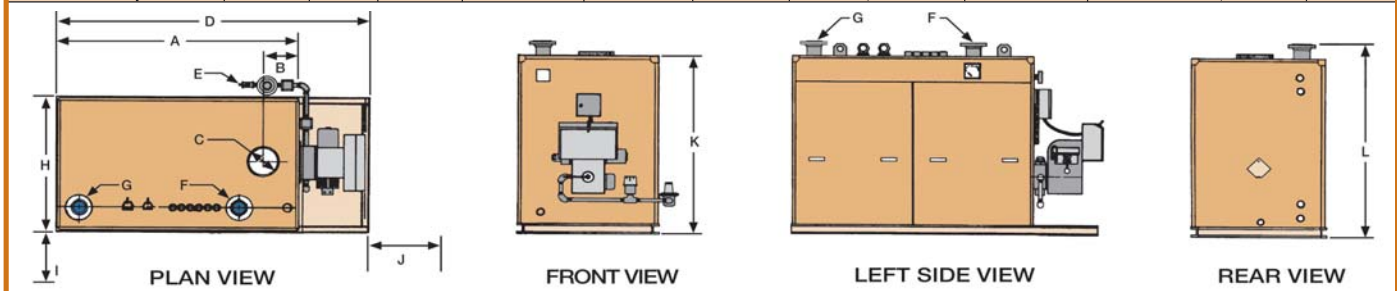
HOT WATER HEATING BOILER DIMENSIONS in inches (cm)
