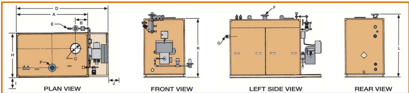
STEAM HEATING/PROCESSING BOILER DIMENSIONS in inches (cm)
